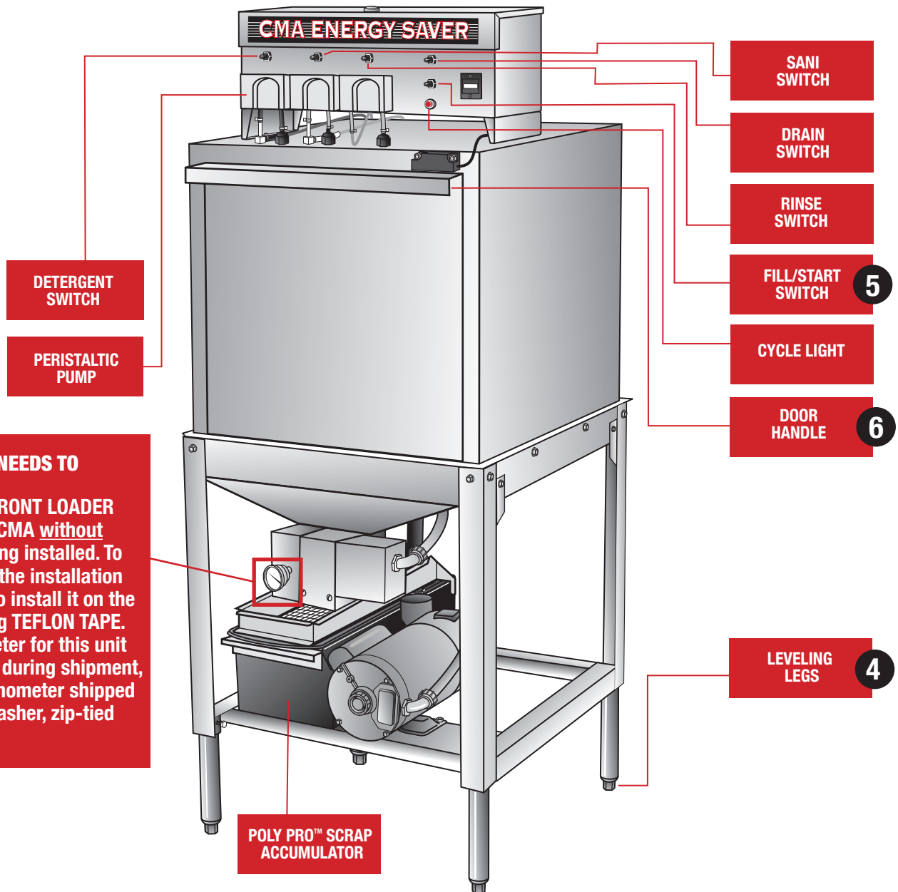
MODEL EST FRONT LOADER FRONT VIEW
