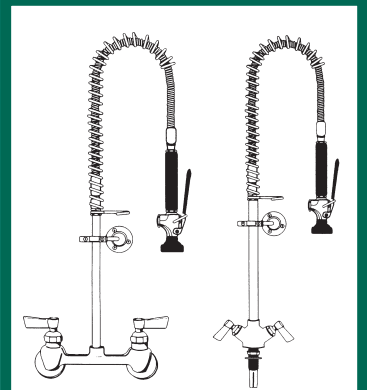
Fisher Pre-Rinse 8" adjustable wall control valve and bracket. 20411.00
